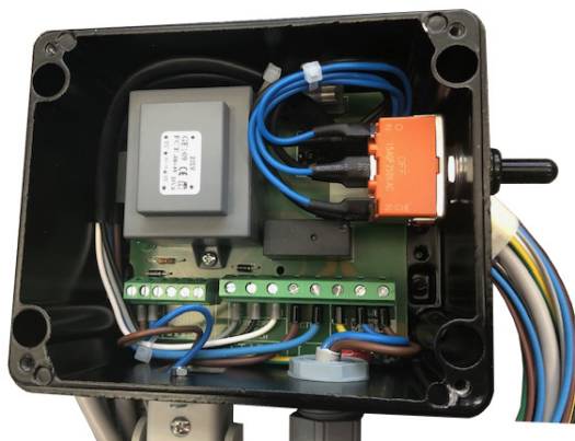
CLAY TARGET THROWING MACHINE IN 230 V. A.C.
