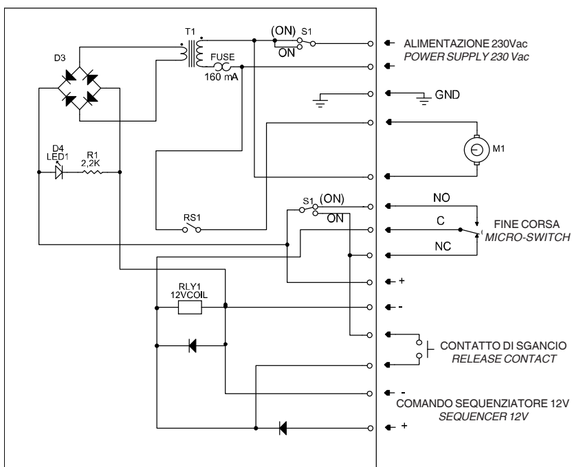
CLAY TARGET THROWING MACHINE IN 230 V. A.C.
